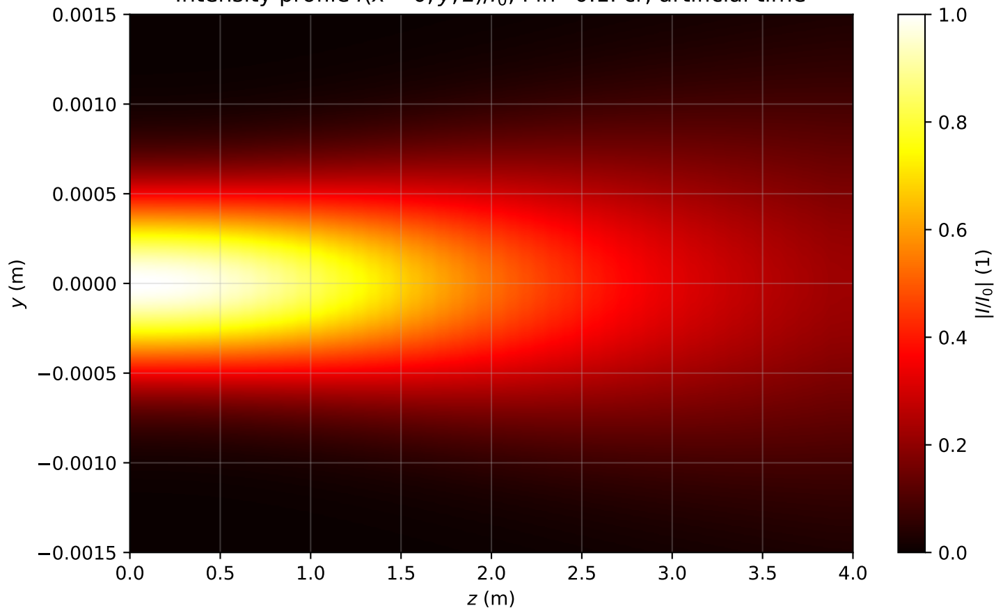
Intensity profile I(x=0, y, z)/I_0 , P_{in}=0.1P_{cr} , artificial time
